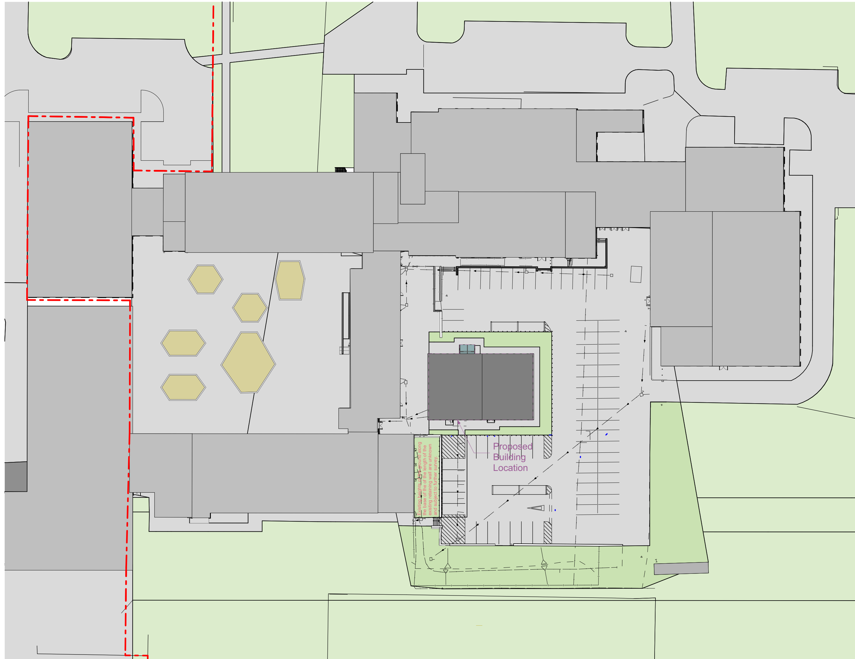
0. Block Plan 1:500
